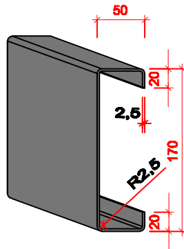
C170.50.2.5
