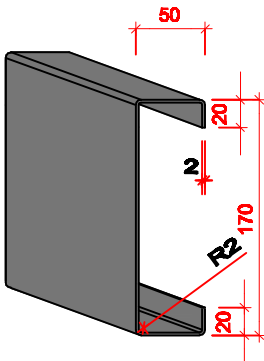
C170.50.2
