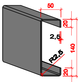
C140.50.2.5
