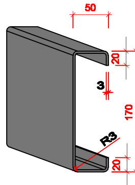
C170.50.3
