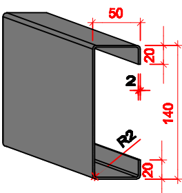
C140.50.2
