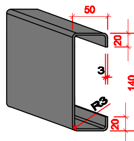
C140.50.3
